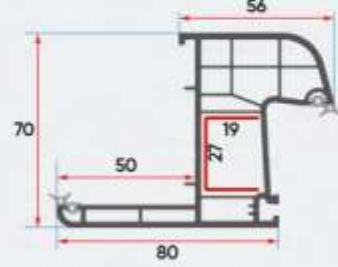
ER 7020 Oval Pervazlı Kasa Profili Ovoid Frame with Cornice Profile
