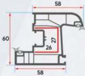
ER 6024 Oval Pencere Kanat Profili Ovoid Window Sash Profile
